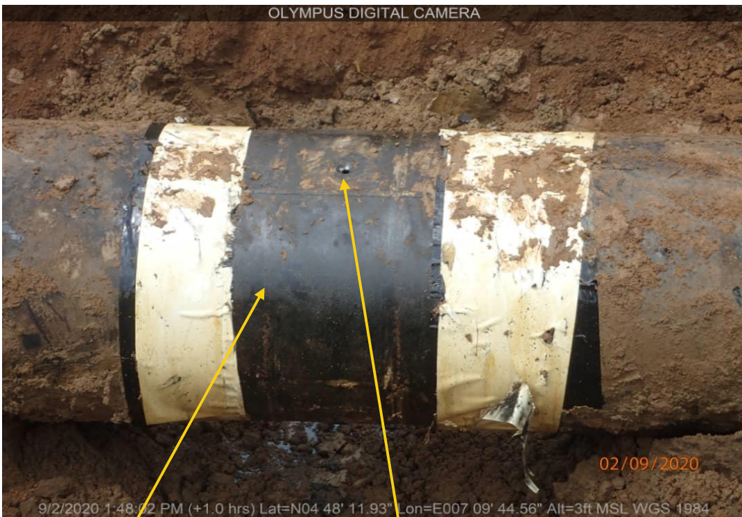
Close-up: Position of missing Clamp and drilled hole at 12 o'clock position on 24" Nkpoku - Bomu Pipeline at Agbeta. Picture was taken during Joint Investigation on 2nd September 2020.
