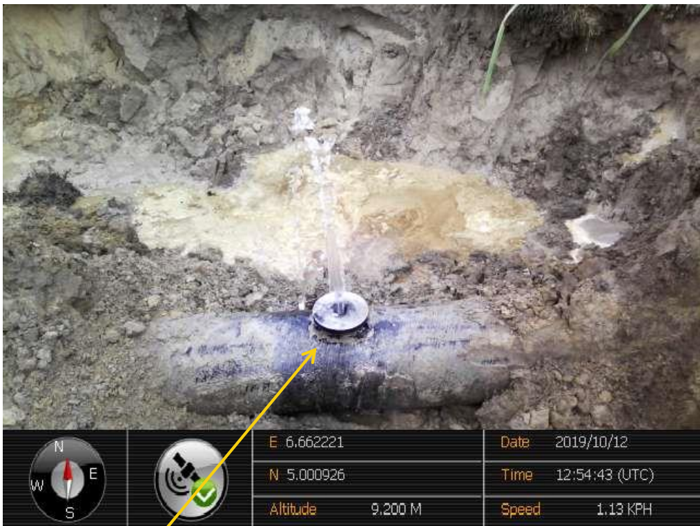
Close-up: Illegal fitting on 14" Okordia - Rumuekpe Pipeline at Ihuowo. Picture was taken during Joint Investigation of 12 th October 2019.
