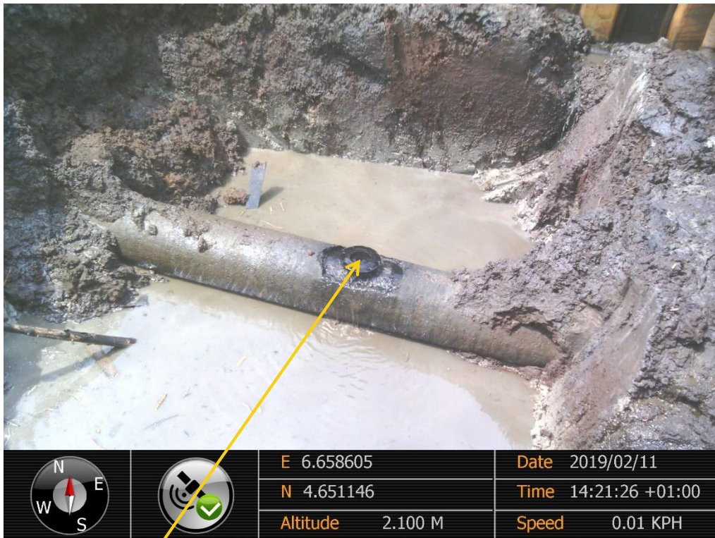
Close-up: Illegal fitting on 18" Soku – Buguma Pipeline at Soku. Picture was taken during Joint Investigation of 11 th February 2019.
