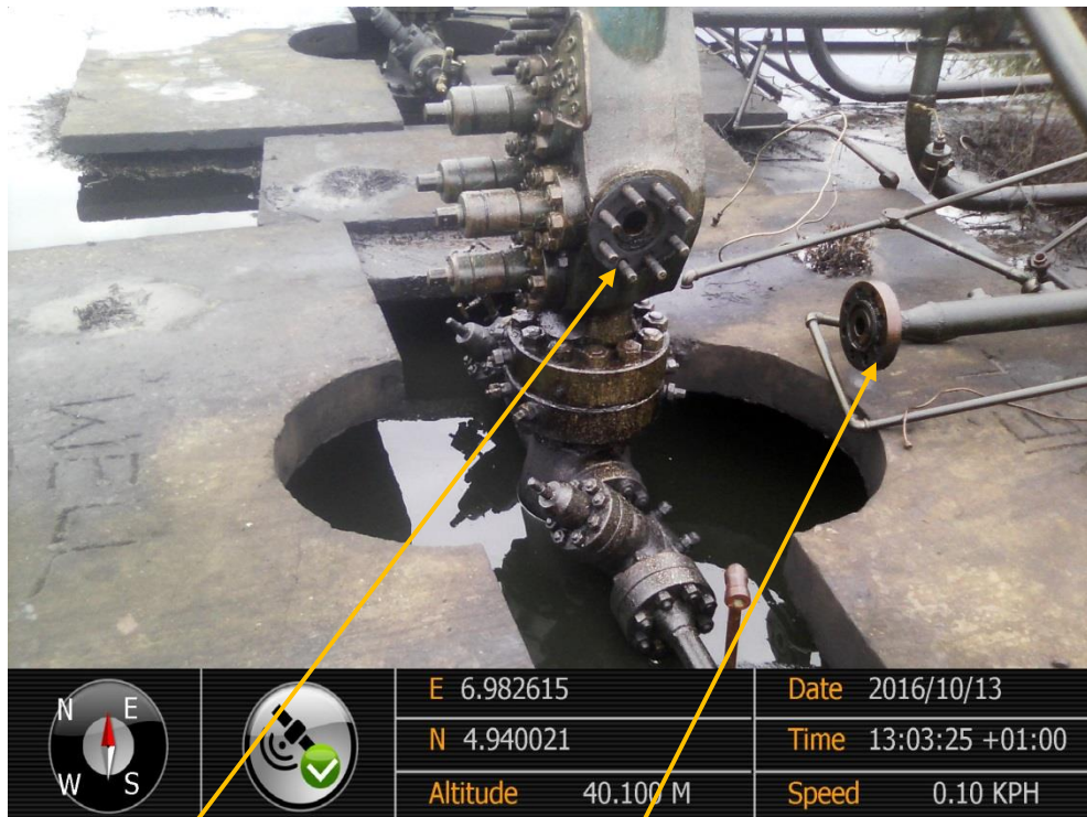
Close-up: Vandalized Wellhead and Disconnected Flowline on Agbada 1 Well 13 and 18 Wellheads at Omunike. Picture was taken during Joint Investigation of 13 th October 2016.
