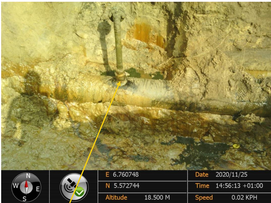
Close-up: 2inch valve illegal connection installed at 12 o'clock position on 12inch Oguta - Egbema Pipeline at Ukwugba. Picture was taken during Joint Investigation on 25th November 2020.
