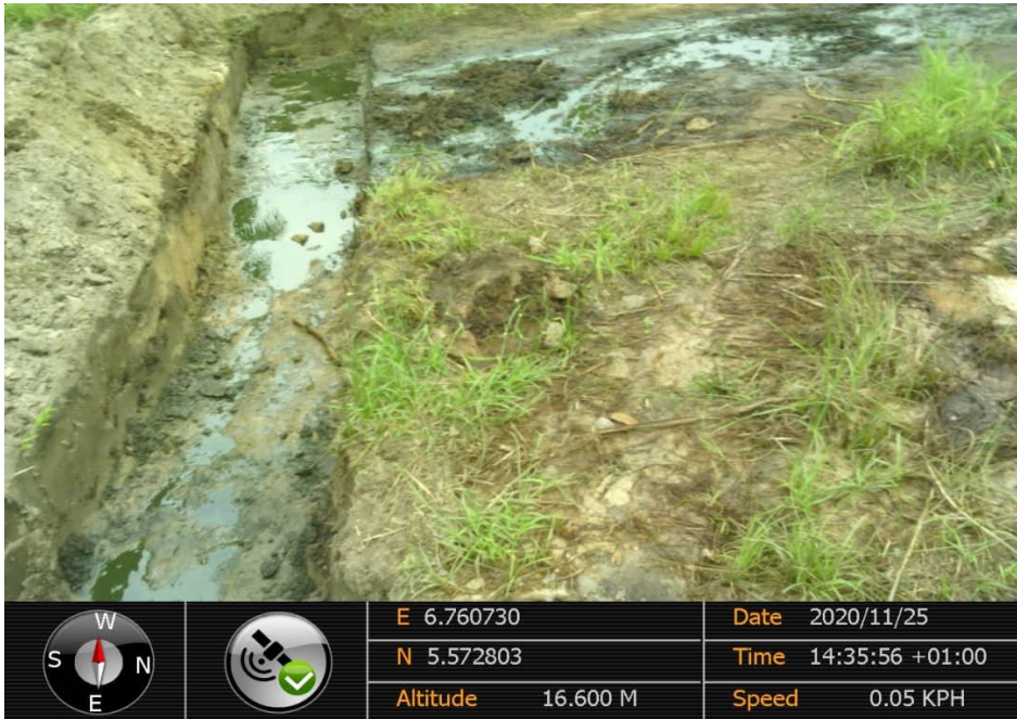
Overview: Part of spill impact on 12inch Oguta Egbema Pipeline at Ukwugba. Picture was taken during Joint Investigation on 25th November 2020.
