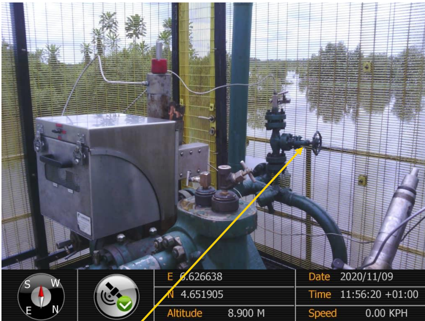
Close-up: Partially closed kerotex valve on Soku Well 14L at Soku. Picture was taken during Joint Investigation on 9 th November 2020.
