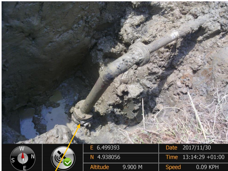
Close-up: Illegal fitting on 20" Kolocreek-Rumuekpe Pipeline at Odau. Picture was taken during Joint Investigation of 30 th November 2017.
