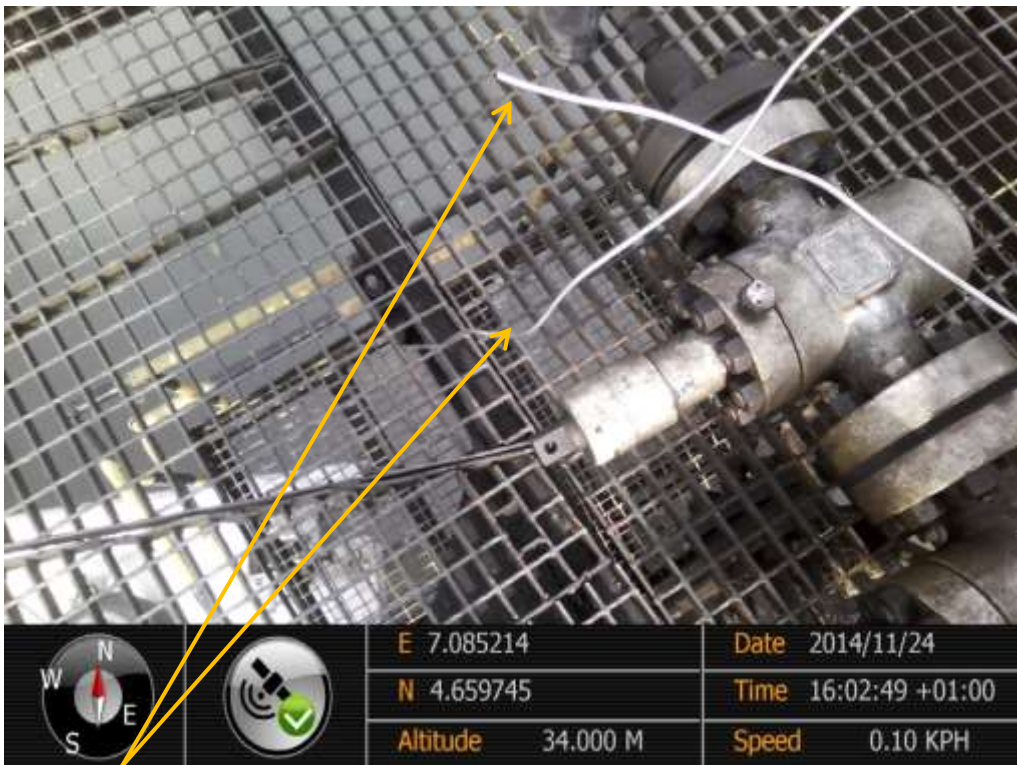
Close-up: Connection points to missing Cameron Control Unit on Alakiri Well31L Wellhead at Ofiomina-Ama. Picture was taken during Joint Investigation of 24 th November 2014.
