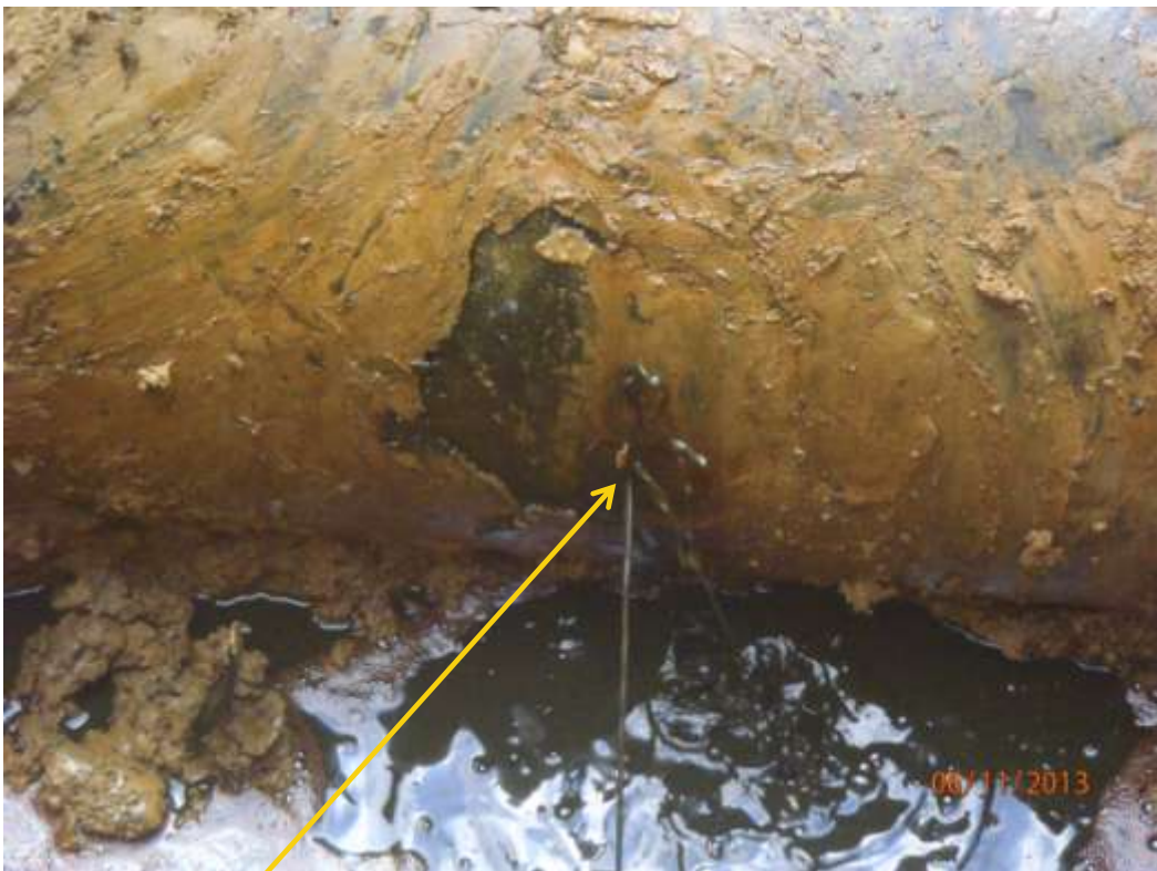
Close-up: Hacksaw cut on 14" Okordia-Rumuekpe Pipeline at Ikarama. Picture was taken during Joint Investigation of 6 th November 2013.
