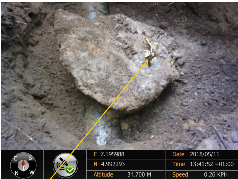
Close-up: Illegal fitting partly concealed in cast concrete on 6" Imo River Well 59T Flowline at Igiriukwu_Owaza. Picture was taken during Joint Investigation of 11 th May 2018.
