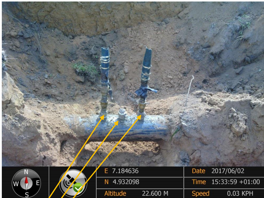
Close-up: Illegal fittings on 12"Imo River-Ogale Pipeline at Okohia-Asa. Picture was taken during Joint Investigation of 2 nd June 2017.
