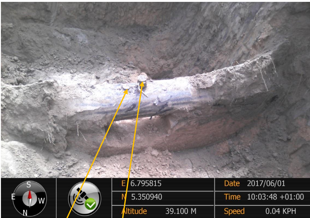
Close-up: 3" non leaking and leaking illegal fitting on 18" Assa-Rumuekpe Pipeline at Ochia. Picture was taken during Joint Investigation of 1 st June 2017.
