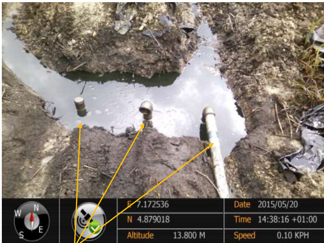
Close-up: Illegal fittings on 12" Imo River – Ogale Pipeline at Komkom. Picture was taken during Joint Investigation of 20 th May 2015.
