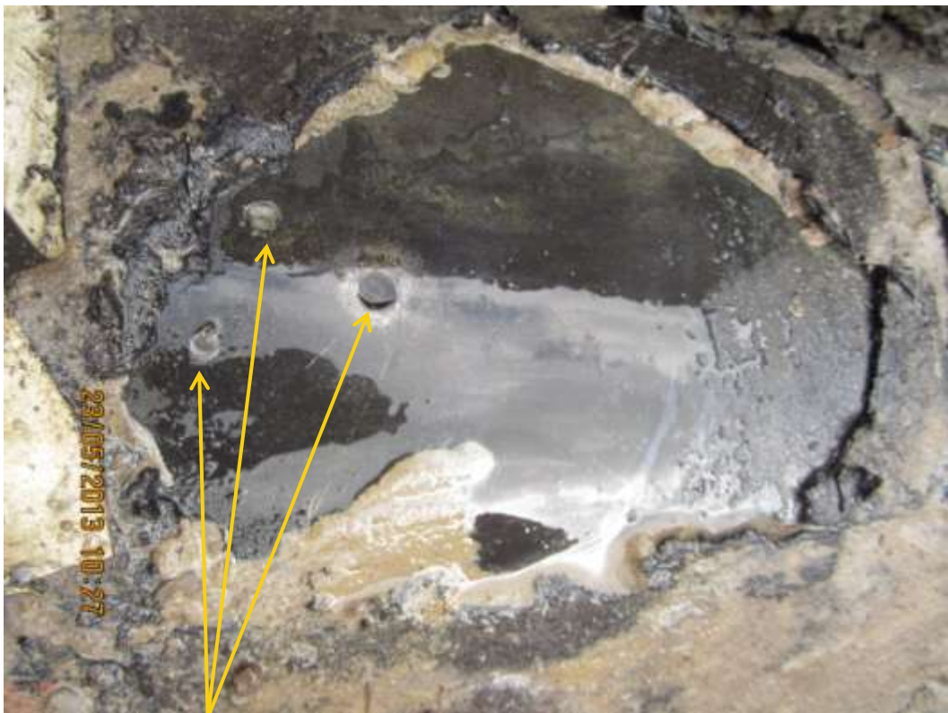
Close up: Drilled holes on 12" Oguta-Egbema pipeline at Obiakpu. Picture was taken during Joint Investigation of 23 rd May 2013.
