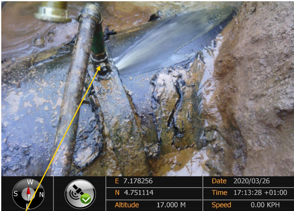
Close-up: 1" valve installed at 12 o'clock position on 28" Nkpoku Bomu Pipeline at Eteo. Picture was taken during Joint Investigation of 26 th March 2020.
