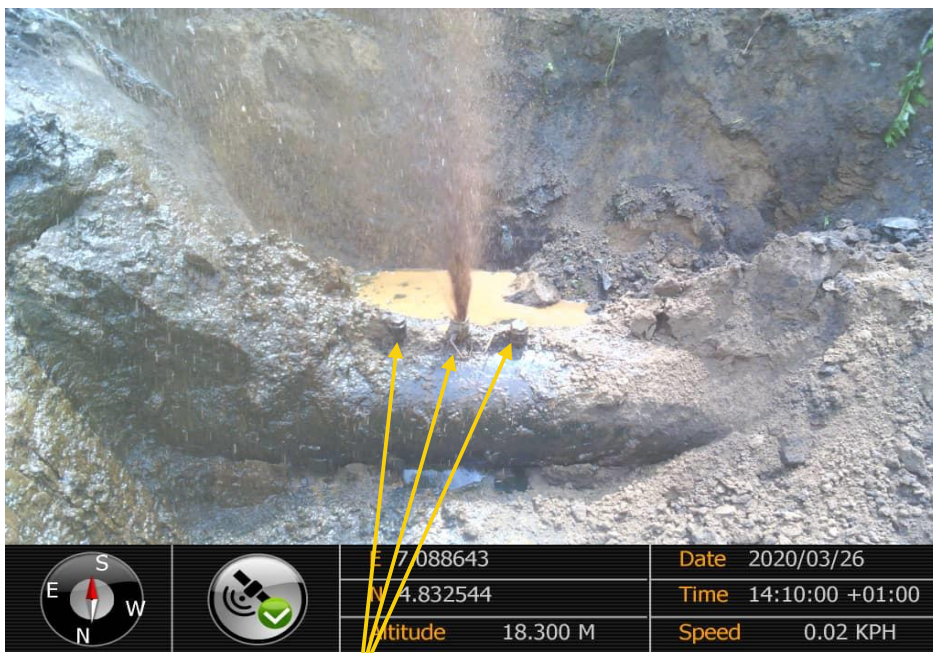
Close-up: 2'' valve crude oil theft points installed at 12 o'clock position on 28'' Nkpoku - Bomu Pipeline at Akpajo. Picture was taken during Joint Investigation of 26 th March 2020.
