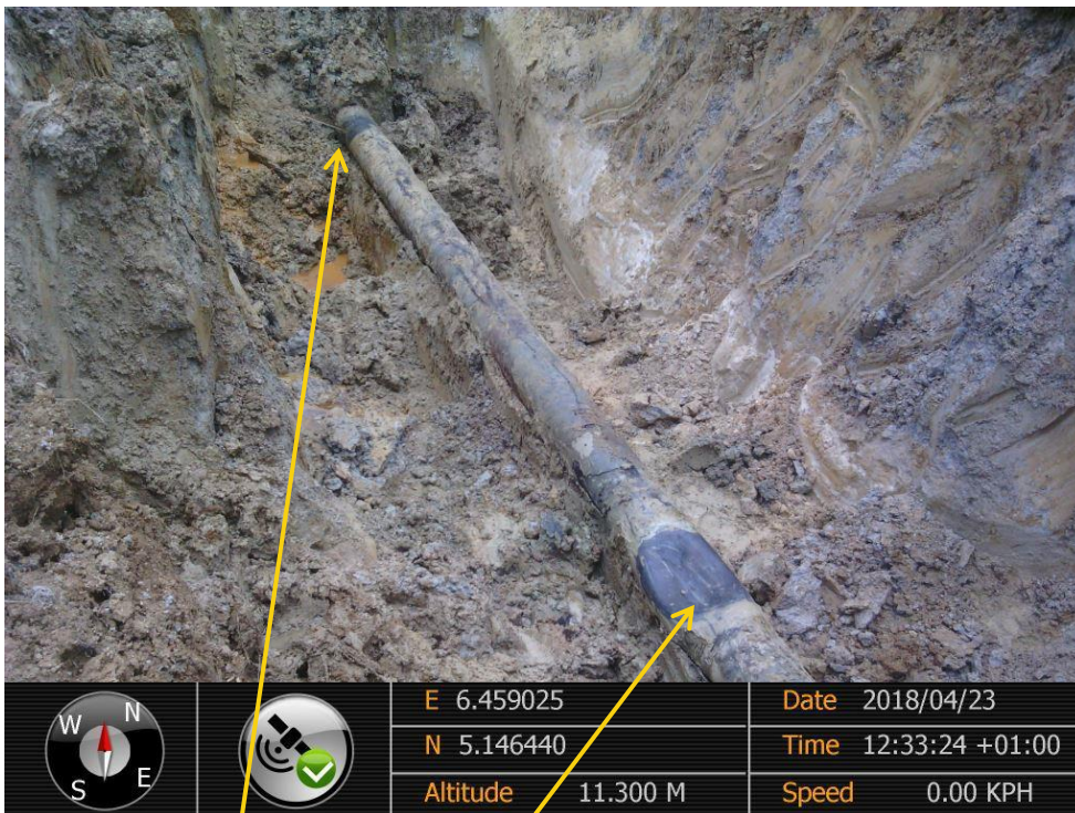
Close-up: Hacksaw Cut and Inward dent on 14" Okordia-Rumuekpe Pipeline at Ikarama. Picture was taken during Joint Investigation of 23 rd April 2018.
