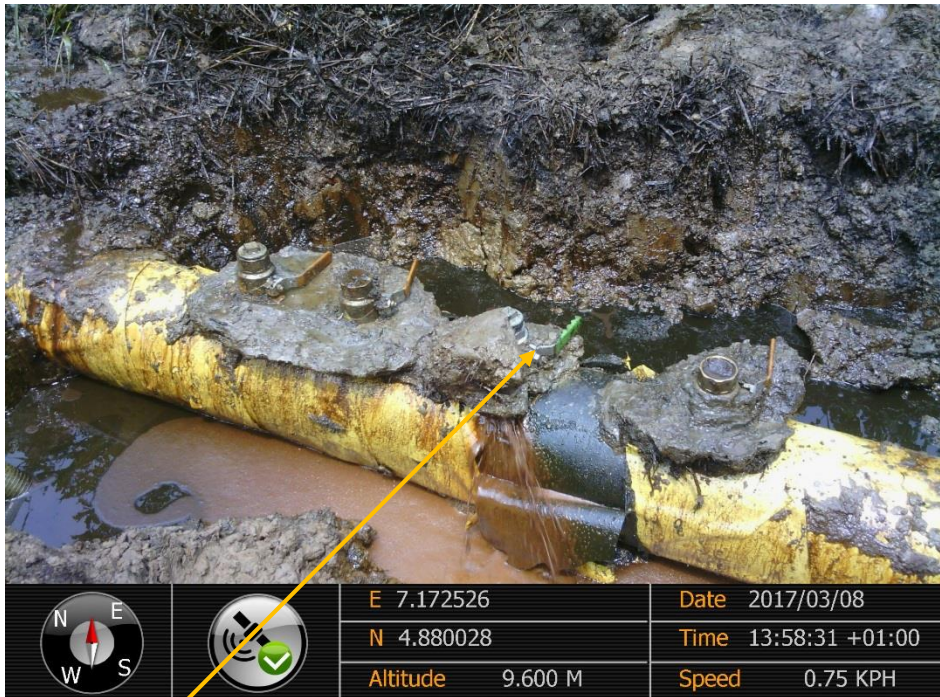
Close-up: Leaking Illegal fitting on 12" Imo River-Ogale Pipeline at Komkom. Picture was taken during Joint Investigation of 8 th March 2017.
