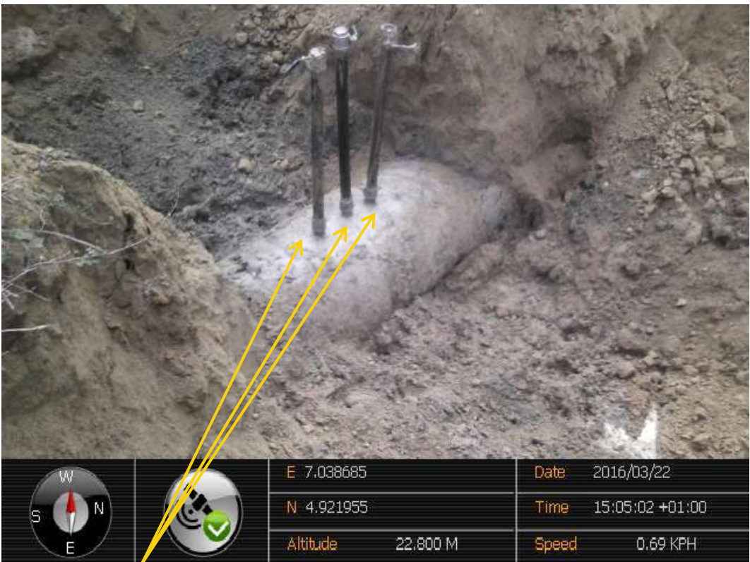
Close-up: Illegal fittings on 36" Nkpoku-Bomu Trans Niger Pipeline at Rumuchiolu/Eneka. Picture was taken during Joint Investigation of 22 nd March 2016.
