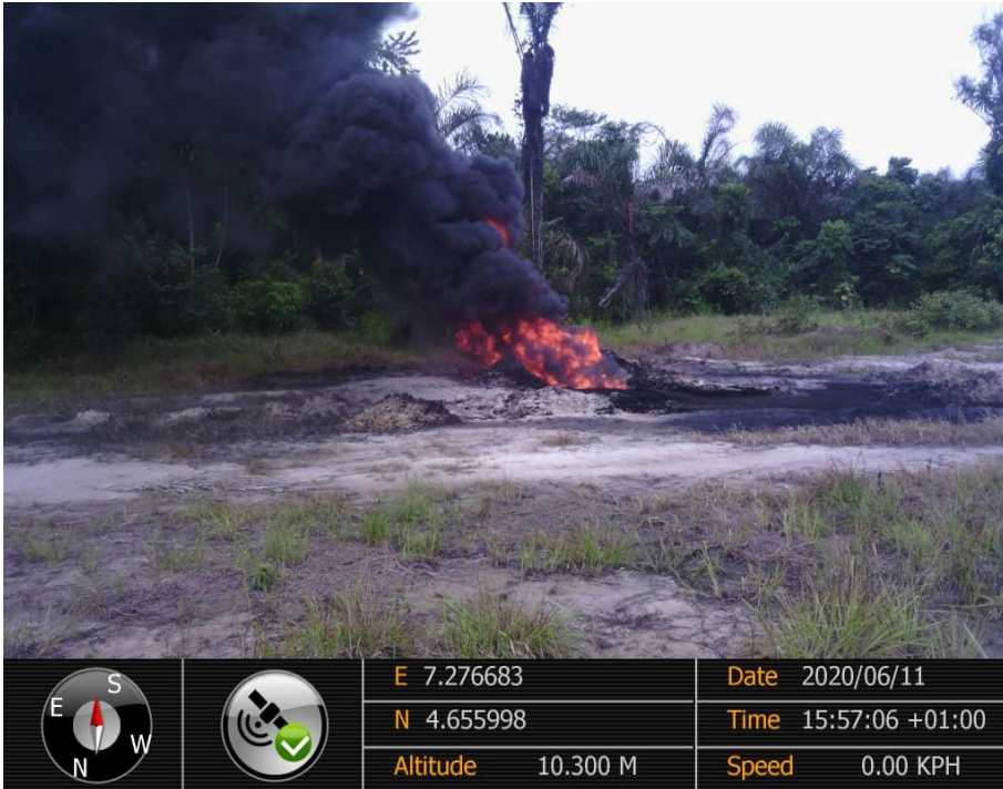
Overview: Part of spill impact on 28" Bomu Bonny Pipeline at Kpor. Picture was taken during Joint Investigation of 11 th June 2020.
