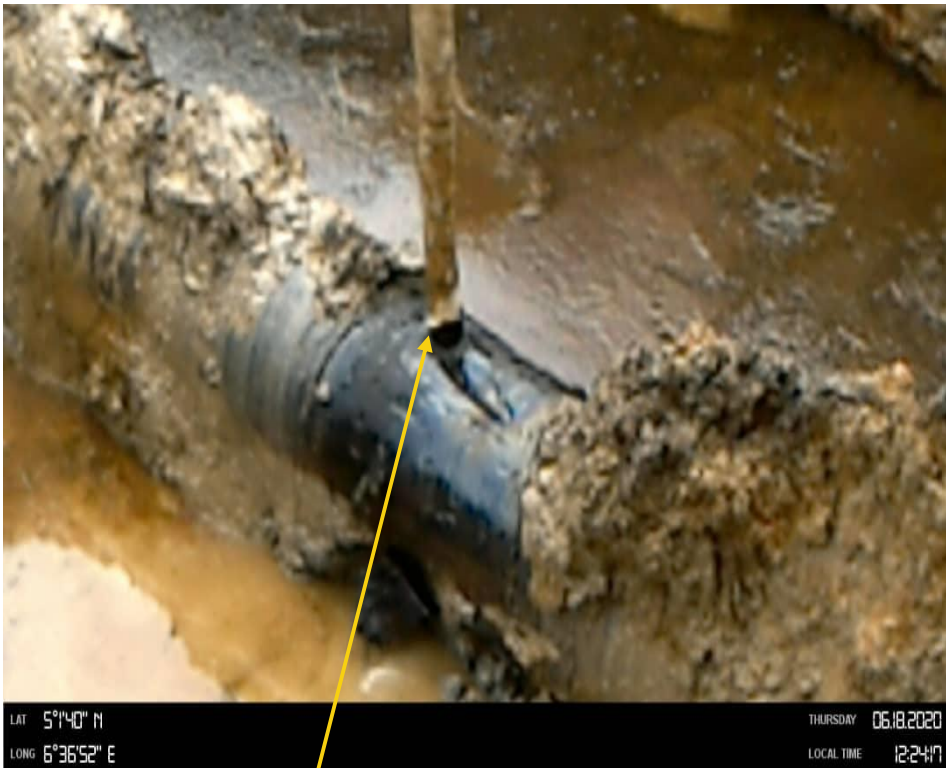
Close-up: Plugged Crude Oil theft point installed at 12 o'clock position on 14" Okordia Rumuekpe Pipeline at Edeoha. Picture was taken during Joint Investigation 18th June 2020.
