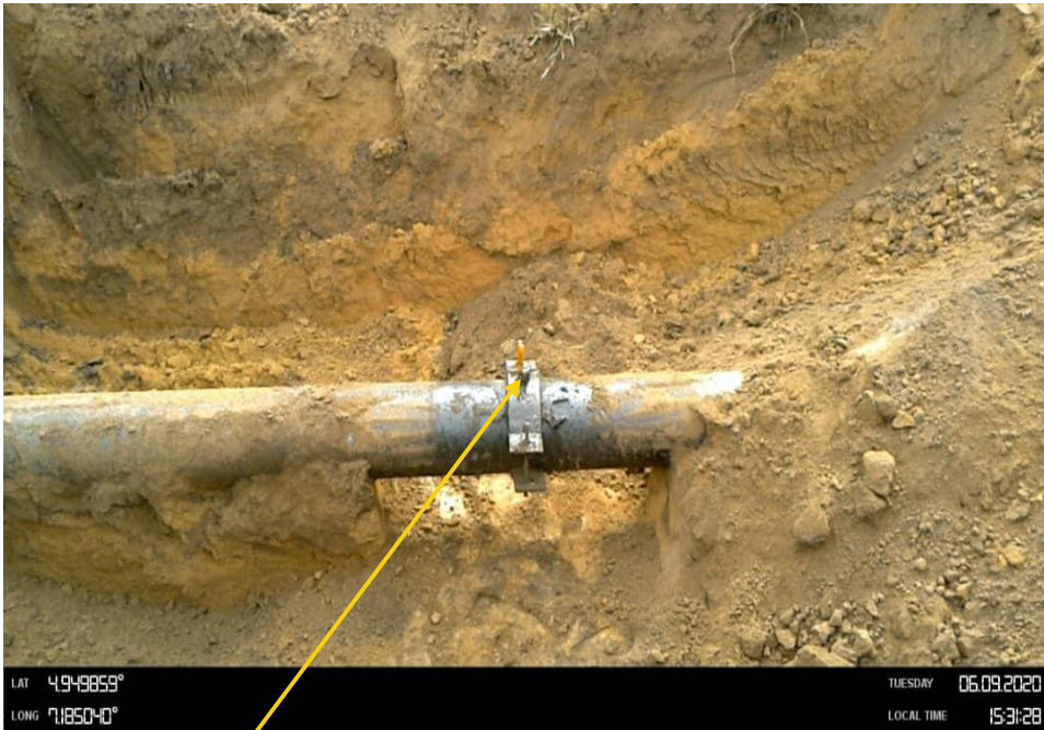
Close-up: 2" Crude oil theft valve on a locally fabricated clamp on 12" Imo River - Ogale Pipeline at Umuololo . Picture was taken during Joint Investigation 9th June 2020.
