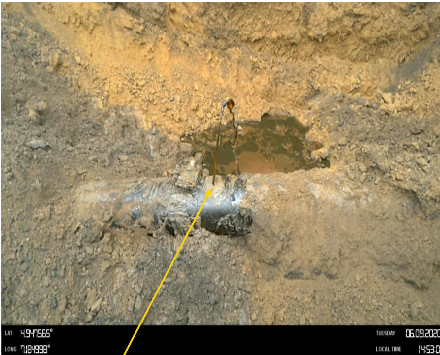
Close-up: 3mm Drilled hole at 12 o'clock position on 12" Imo River - Ogale Pipeline at Umuololo . Picture was taken during Joint Investigation 9th June 2020.
