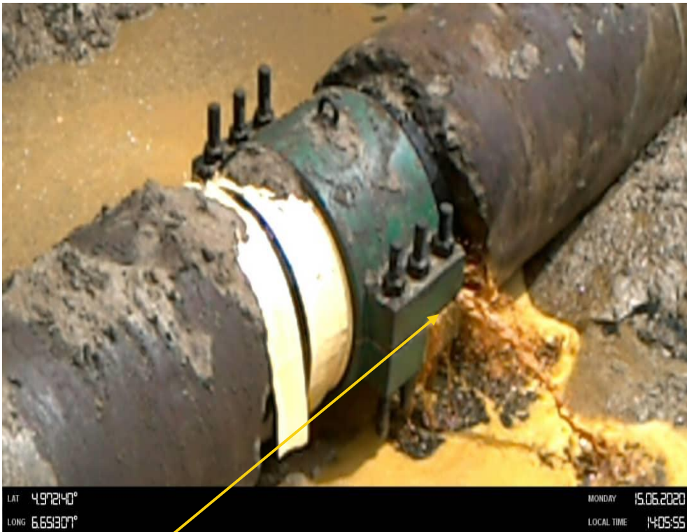
Close-up: Tampered clamp on New 20'' Kolocreek - Rumuekpe Pipeline at Okoma 1 . Picture was taken during Joint Investigation 15 th June 2020
