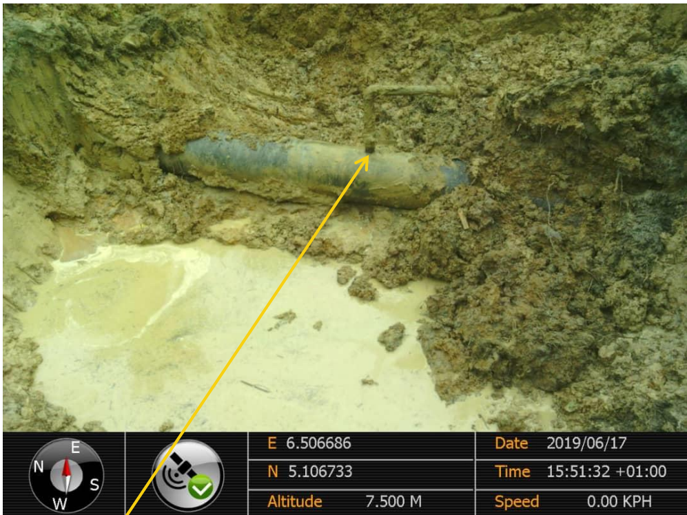
Close-up: Illegal Fitting on 14" Okordia – Rumuekpe Pipeline at Oshie. Picture was taken during Joint Investigation of 17 th June 2019
