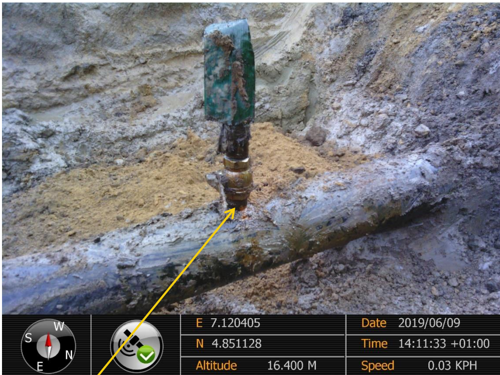
Close-up: Illegal fitting on 8'' Obigbo North – New Elenwa Pipeline at Umusonaya. Picture was taken during Joint Investigation of 9 th June 2019
