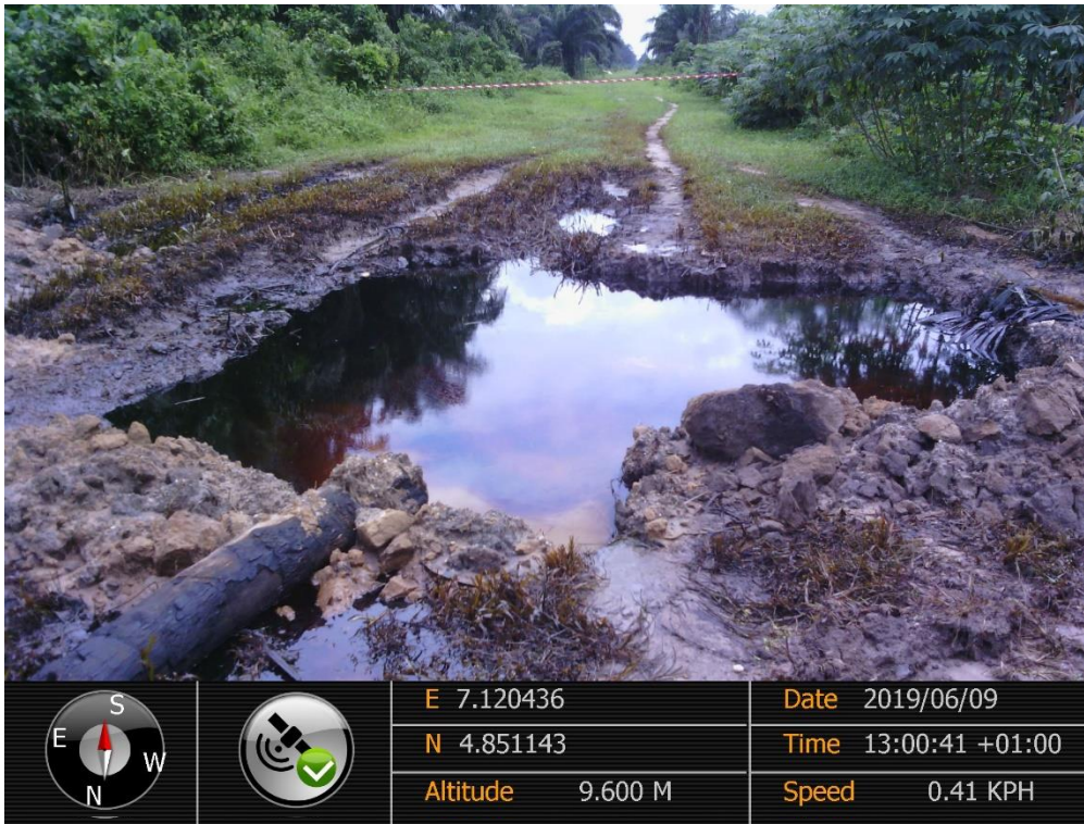
Overview: Part of spill impact on 8'' Obigbo North – New Elenwa Pipeline Right of Way at Umusonaya. Picture was taken during Joint Investigation of 9 th June 2019.
