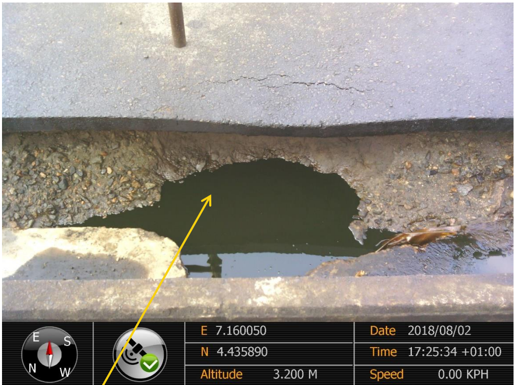
Close-up: Crude oil seeping from ground on 16" Bonny Disused Export Pipelines at Bonny. Picture was taken during Joint Investigation of 2 nd August 2018.
