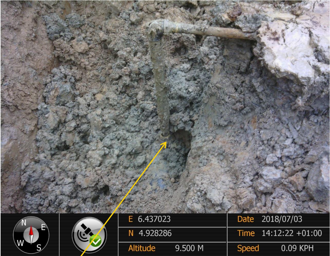
Close-up: Illegal Fitting on 20" Kolocreek-Rumuekpe Pipeline at Odau KM9. Picture was taken during Joint Investigation of 3 rd July 2018.
