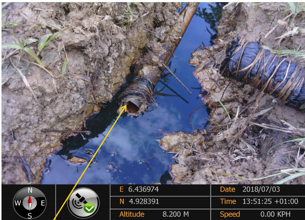
Close-up: Leak point from 2" pipe extension on 20" Kolocreek-Rumuekpe Pipeline at Odau KM9. Picture was taken during Joint Investigation of 3 rd July 2018.
