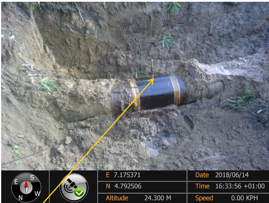
Close-up: Illegal fitting on 24" Nkpoku-Bomu Pipeline at Egbalor. . Picture was taken during Joint Investigation of 14 th June 2018.
