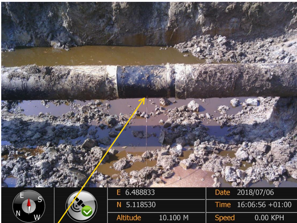
Close-up: Drilled Hole on 14" Okordia-Rumuekpe Pipeline at Akaramini . Picture was taken during Joint Investigation of 6 th July 2018.
