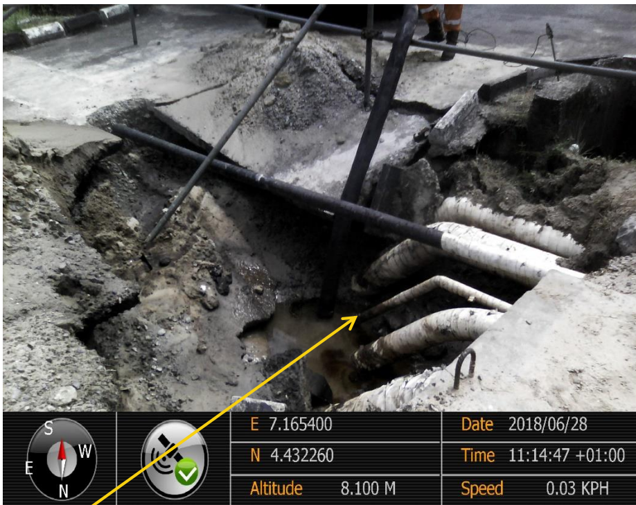
Close-up: Corrosion on 2" BNAG-Incoming Manifold Condensate Line at Bonny. Picture was taken during Joint Investigation of 28 th June 2018.
