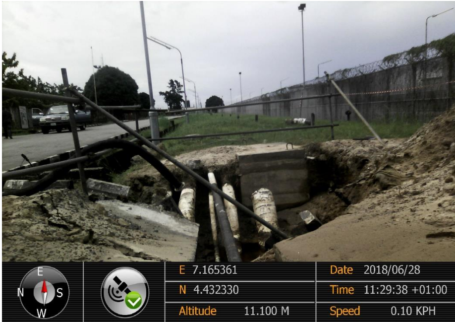
Overview: Part of spill impact on 2" BNAG-Incoming Manifold Condensate Line at Bonny. Picture was taken during Joint Investigation of 28 th June 2018.
