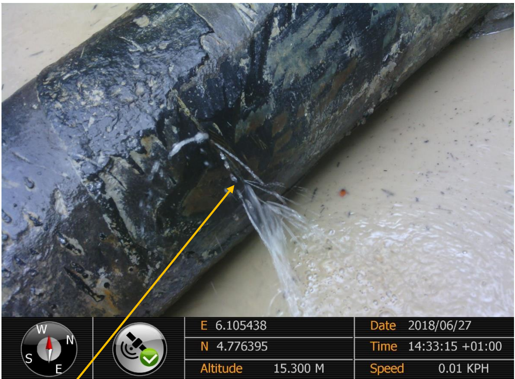
Close-up: Hacksaw Cut on 10'' DiebuCreek– Nun River Pipeline at Oporoma. Picture was taken during Joint Investigation of 27 th June 2018.
