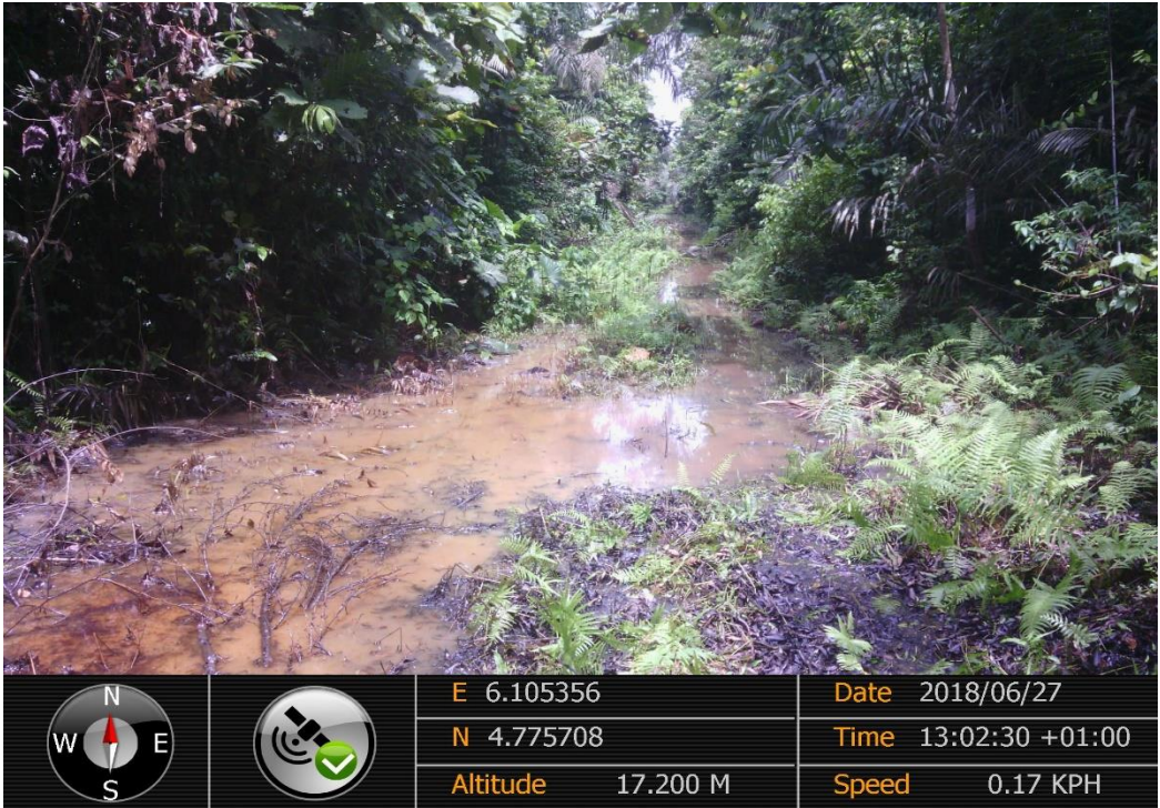
Overview: Part of spill impact on 10'' DiebuCreek– Nun River Pipeline Right of Way at Oporoma. Picture was taken during Joint Investigation of 27 th June 2018..
