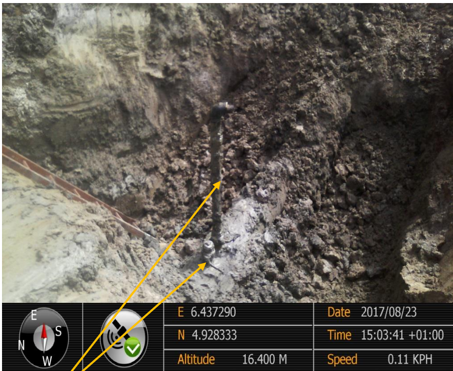
Close-up: Illegal fittings on 20" Kolocreek-Rumuekpe Pipeline at Odau. Picture was taken during Joint Investigation of 23 rd August 2017.
