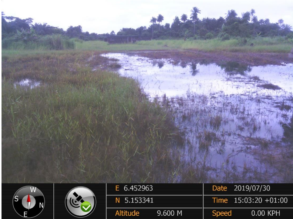
Overview: Part of spill impact on 14" Okordia - Rumuekpe Pipeline Right of Way at Ikarama. Picture was taken during Joint Investigation of 30 th July 2019.
