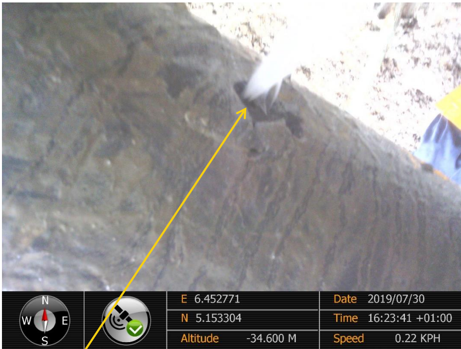
Close-up: Internal Corrosion on 14" Okordia - Rumuekpe Pipeline at Ikarama. Picture was taken during Joint Investigation of 30 th July 2019
