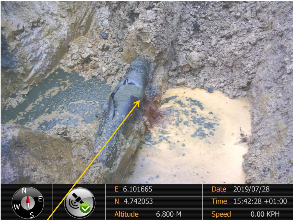
Close-up: Bomb Blast on 10" Diebu – NunRiver Pipeline at Onyoma-Ekowe. Picture was taken during Joint Investigation of 28 th July 2019
