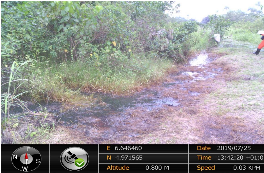
Overview: Part of spill impact on 20'' Kolocreek - Rumuekpe Pipeline Right of Way at Okoma. Picture was taken during Joint Investigation of 25 th July 2019.
