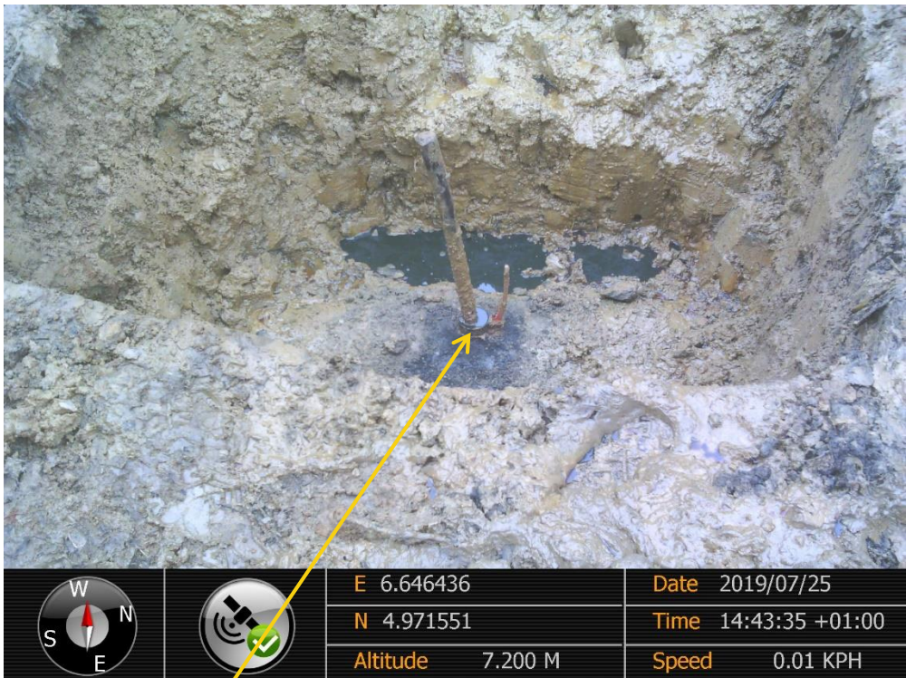
Close-up: Plugged Illegal fitting on 20'' Kolocreek - Rumuekpe Pipeline at Okoma. Picture was taken during Joint Investigation of 25 th July 2019
