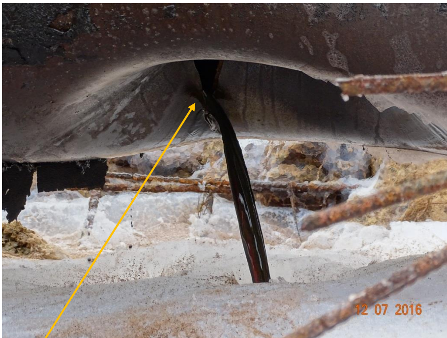
Close-up: Tear/inward dent on 28" Nkpoku - Bomu Pipeline at Gio – Kporghor. Picture was taken during Joint Investigation of 12 th July 2016.
