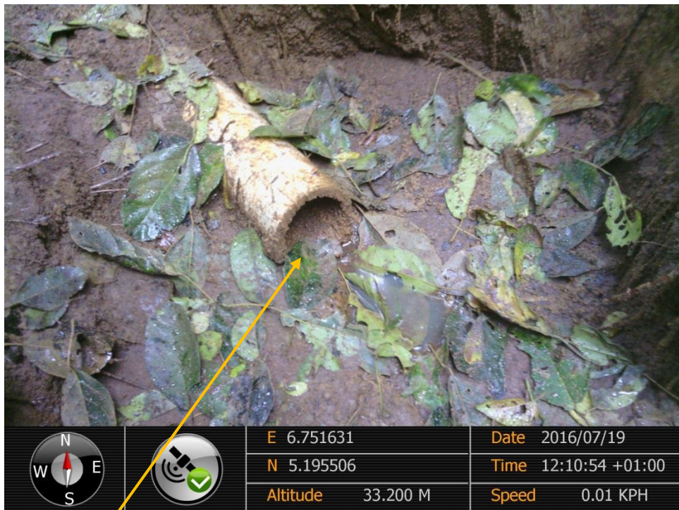
Close-up: Part of Missing Flowline on Ahia Well 3S Flowline at Egbeda. Picture was taken during Joint Investigation of 19 th July 2016.
