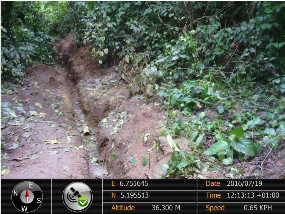
Overview: Part of spill impact on Ahia Well 3S Flowline at Egbeda. Picture was taken during Joint Investigation of 19 th July 2016.
