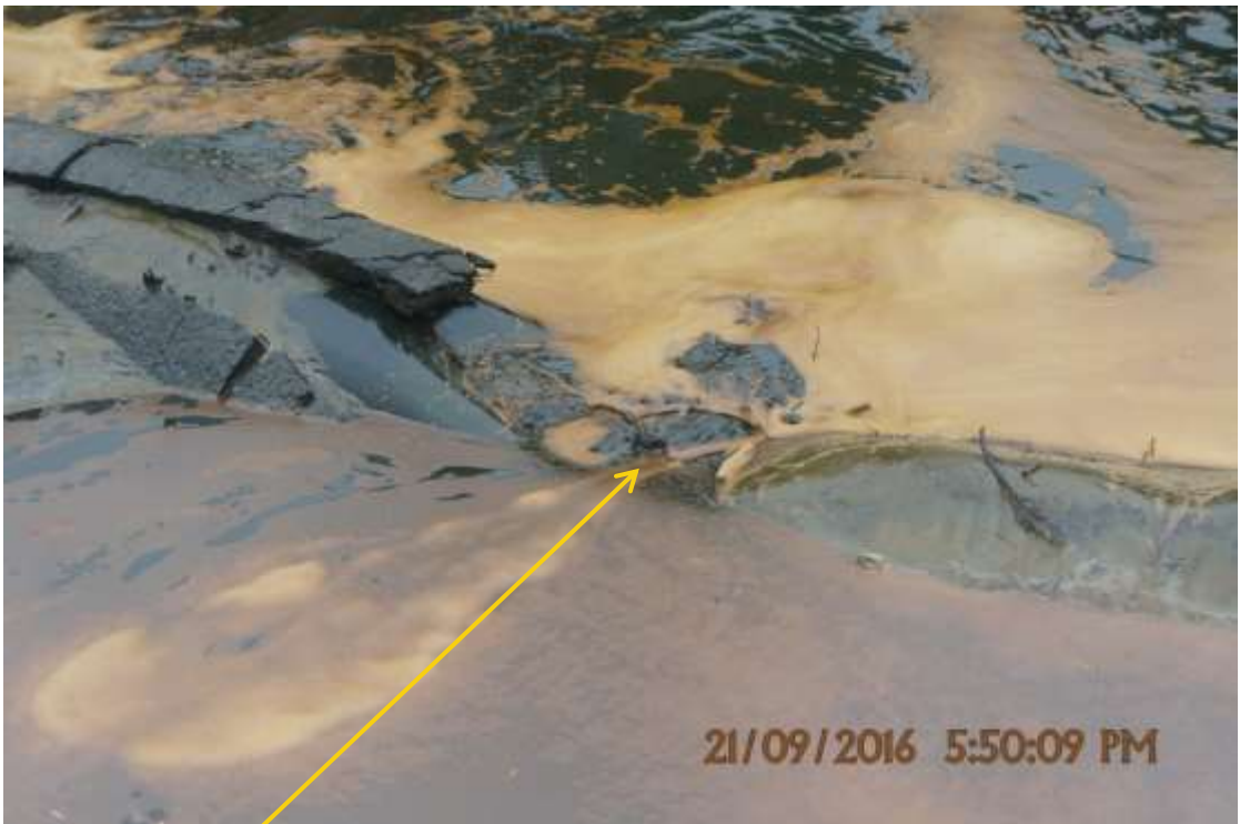
Close-up: Inward dent and tear on 24" Trans Ramos Pipeline at Odimodi. Picture was taken during Joint Investigation of 21 st September 2016.
