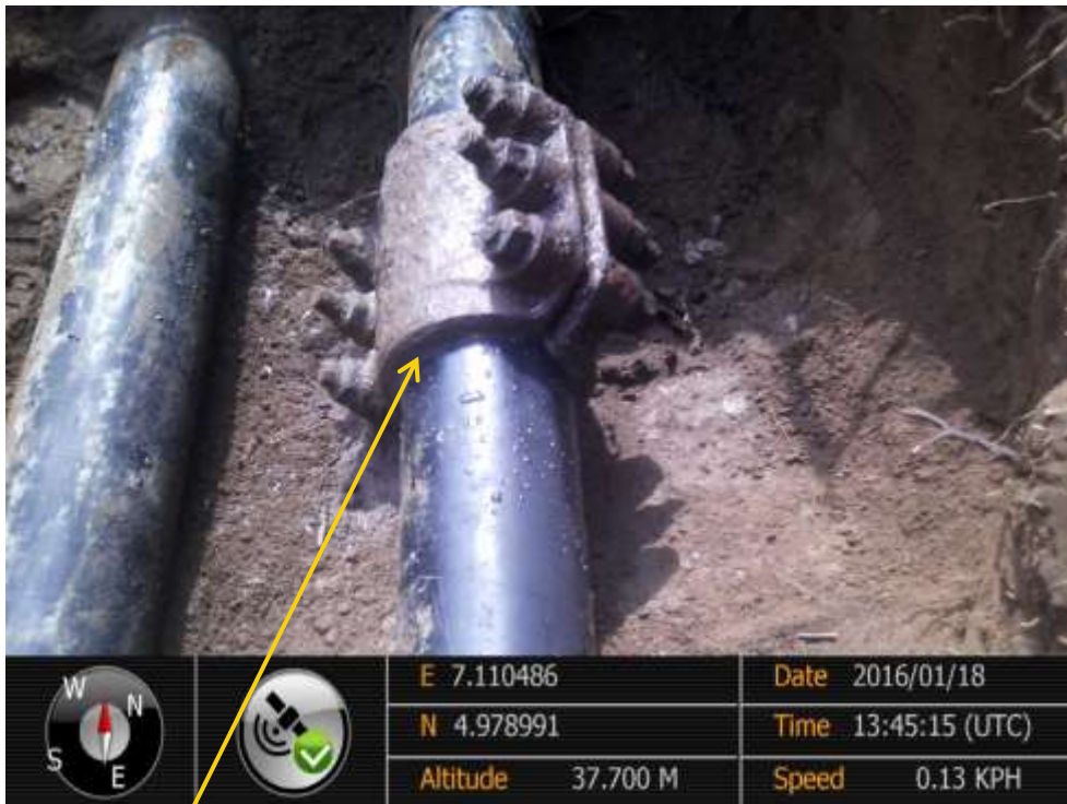
Close-up: Failed clamp on 4" Nkali Well10S Flowline at Odagwa2. Picture was taken during Joint Investigation of 18 th January 2016.
