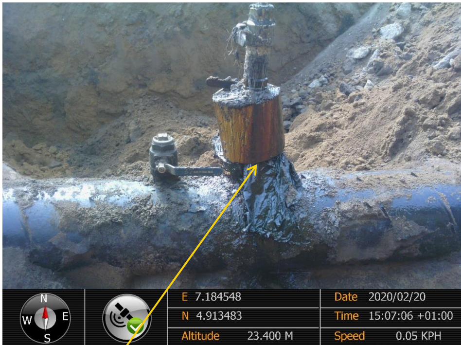
Close-up: Leaking 2" Ball Valve Installed at 12 o'clock position on 12" Imo River1 – Ogale Pipeline at Uzuaku. Picture was taken during Joint Investigation of 20 th February 2020.
