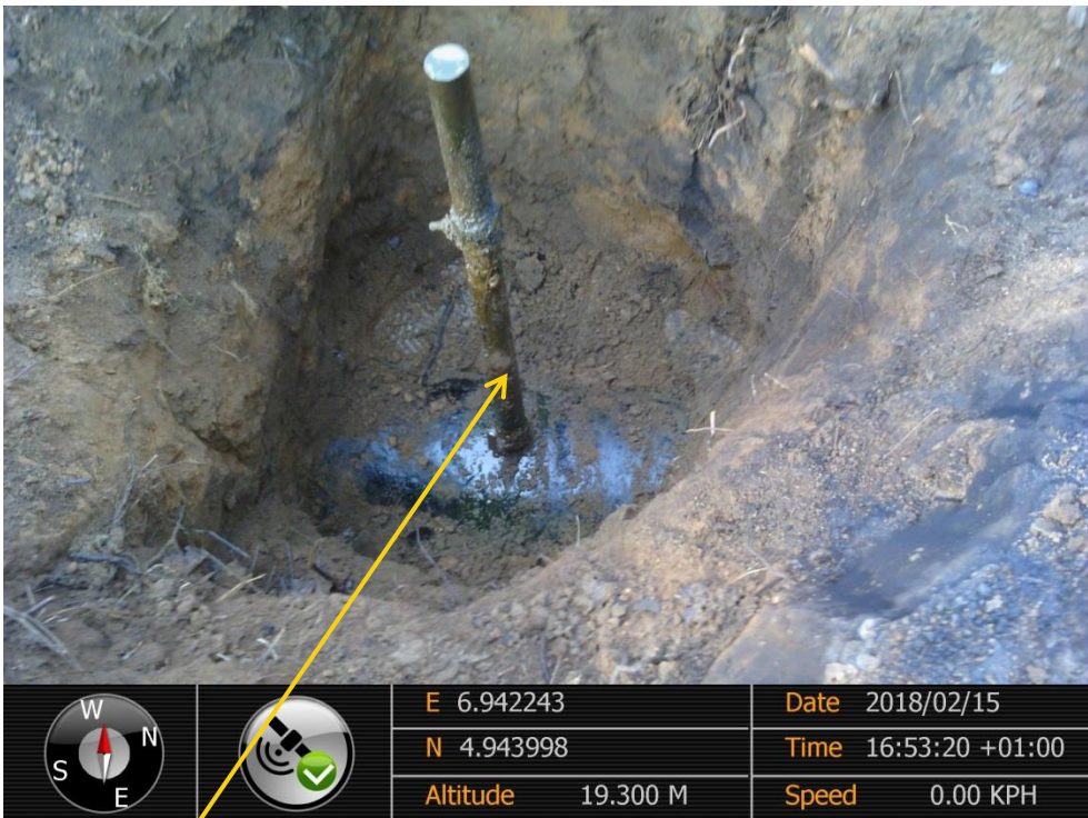
Close-up: Illegal fitting on 20''Rumuekpe-Nkpoku Pipeline at Omuigwe-Aluu. Picture was taken during Joint Investigation of 15 th February 2018.
