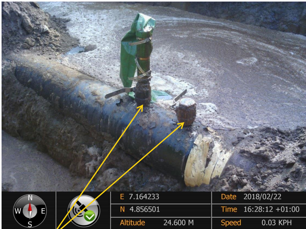
Close-up: Illegal fitting on 12" Imo River – Ogale Pipeline at Kom-Kom. Picture was taken during Joint Investigation of 22 nd February 2018.
