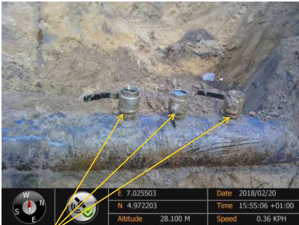
Close-up: Illegal fittings on 8" Umuechem-Nkpoku Pipeline at Omusele. Picture was taken during Joint Investigation of 20 th February 2018.
