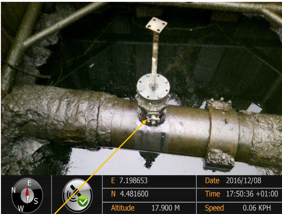
Close-up: Illegal fitting on 28" Bomu-Bonny Pipeline at Okolomabio-Oloma. Picture was taken during Joint Investigation of 8 th December 2016.
