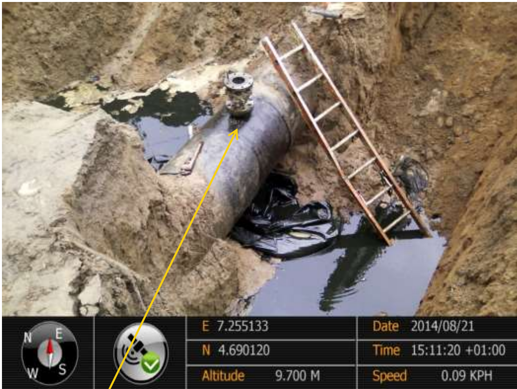
Close-up: Illegal fitting on 28" Nkpoku-Bomu Pipeline Right of Way at B-Dere. Picture was taken during Joint Investigation of 21 st August 2014.
