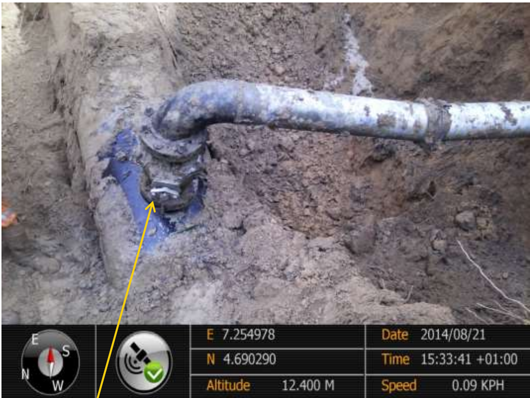
Close-up: Illegal fitting on 28" Nkpoku-Bomu Pipeline at B-Dere. Picture was taken during Joint Investigation of 21 st August 2014.
