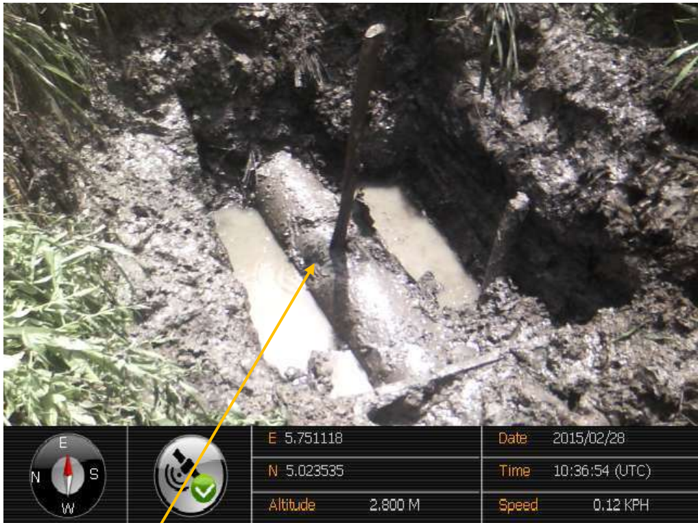
Close-up: Hacksaw cut on 12" Benisede-Isampou Pipeline at Foutorugbene. Picture was taken during Joint Investigation of 28 th February 2015.
