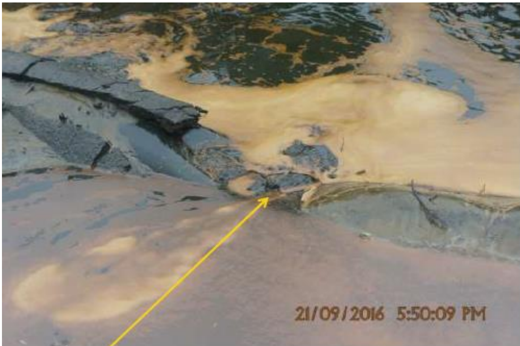
Close-up: Inward dent on 24" Trans Ramos Pipeline at Odimodi. Picture was taken during Joint Investigation of 21 st September 2016.
