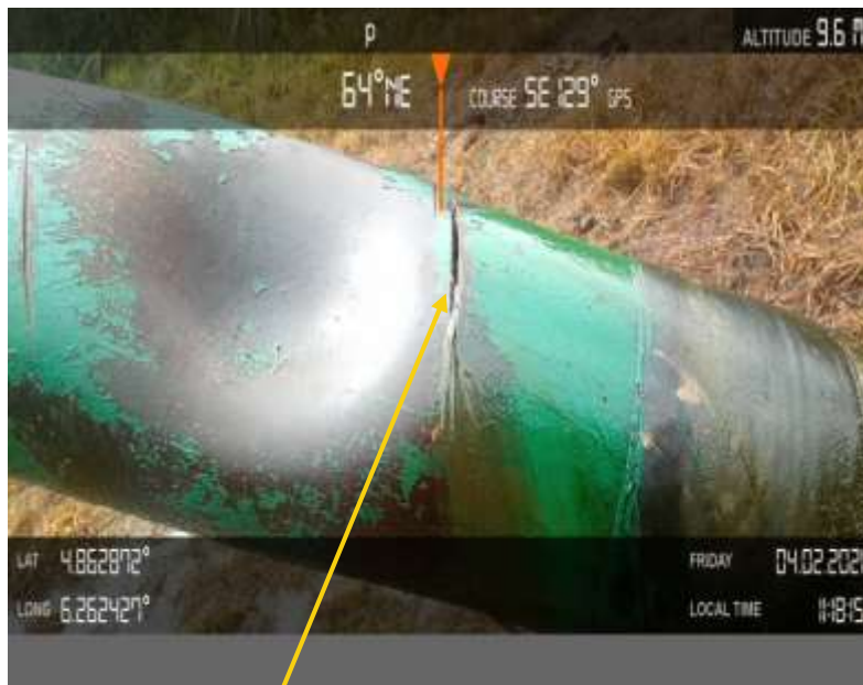
Close-up: Inward dent and Hacksaw cut at 12 o'clock position on 16inch Nun-River Kolocreek BVS riser at Agbura-Otuokpoti. Picture was taken during Joint Investigation of 2 nd April 2021.
