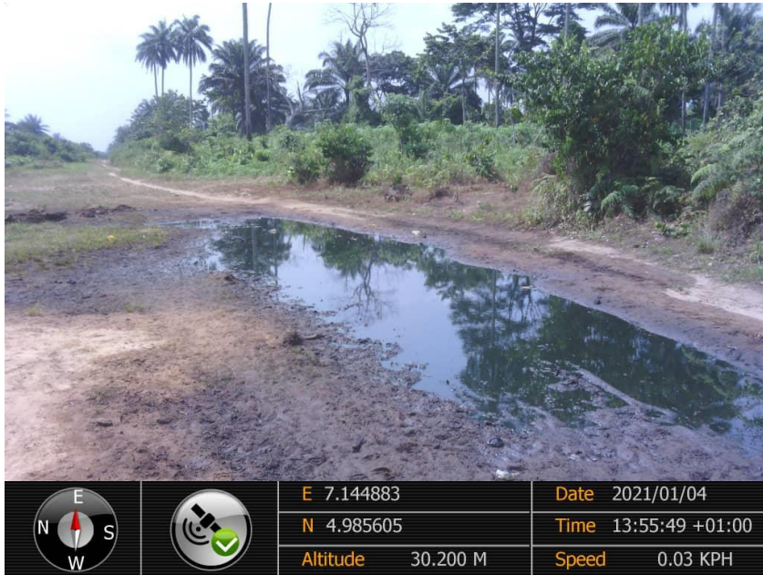
Overview: Part of spill impact on 8" Nkali – Imo River2 Pipeline at Odagwa. Picture was taken during Joint Investigation on 4th January 2021.
