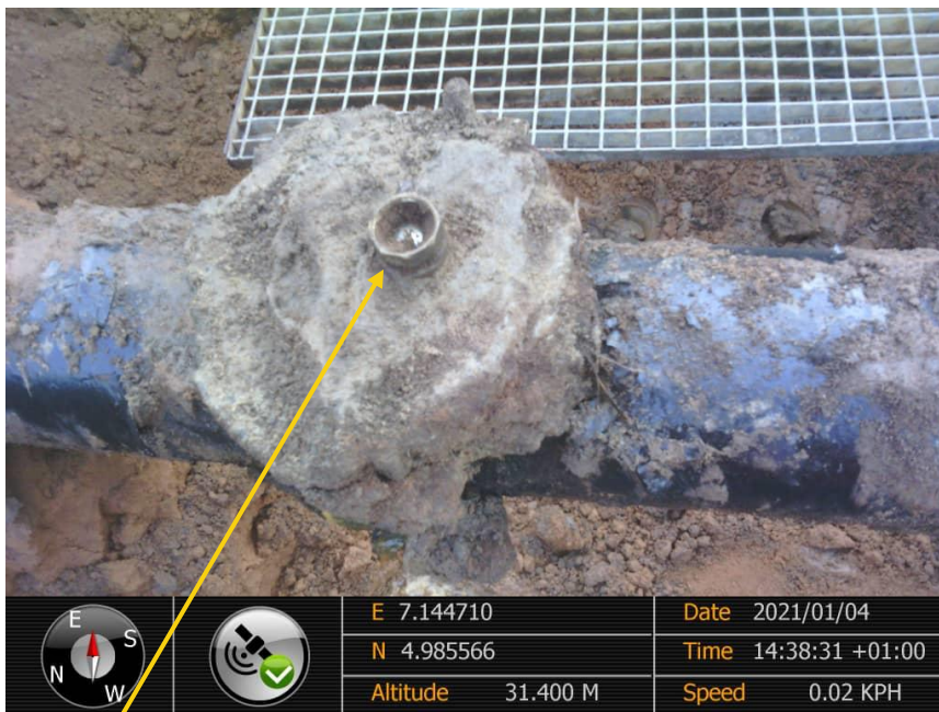
Close-up: 1 inch nipple buried inside a concrete cast at 12 o'clock position on 8" Nkali – Imo River2 Pipeline at Odagwa. Picture was taken during Joint Investigation on 4th January 2021.
